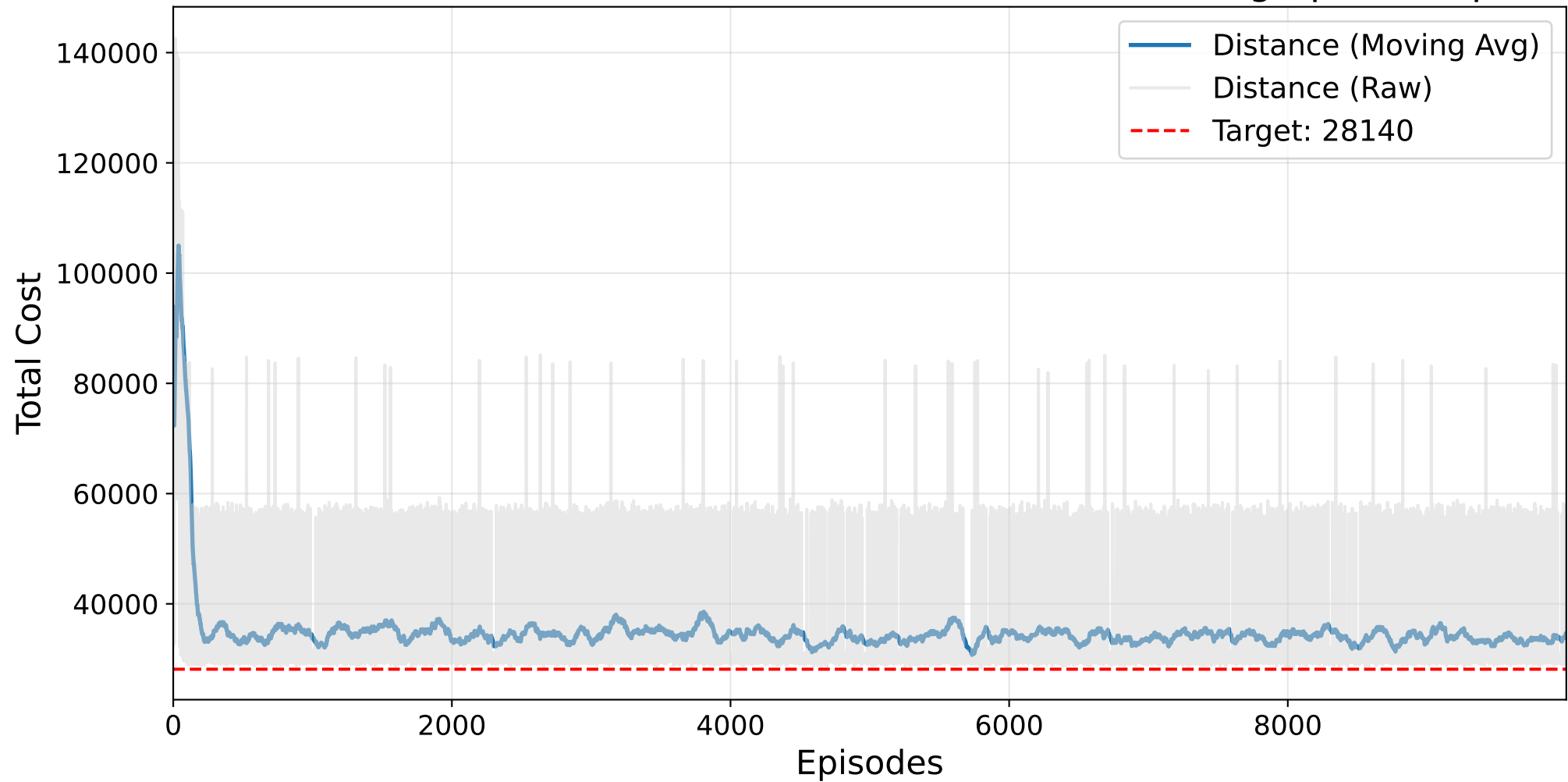
Final GAUSSIAN PROCESS Masked AutoRL-SOP Training - p43.1.sop
